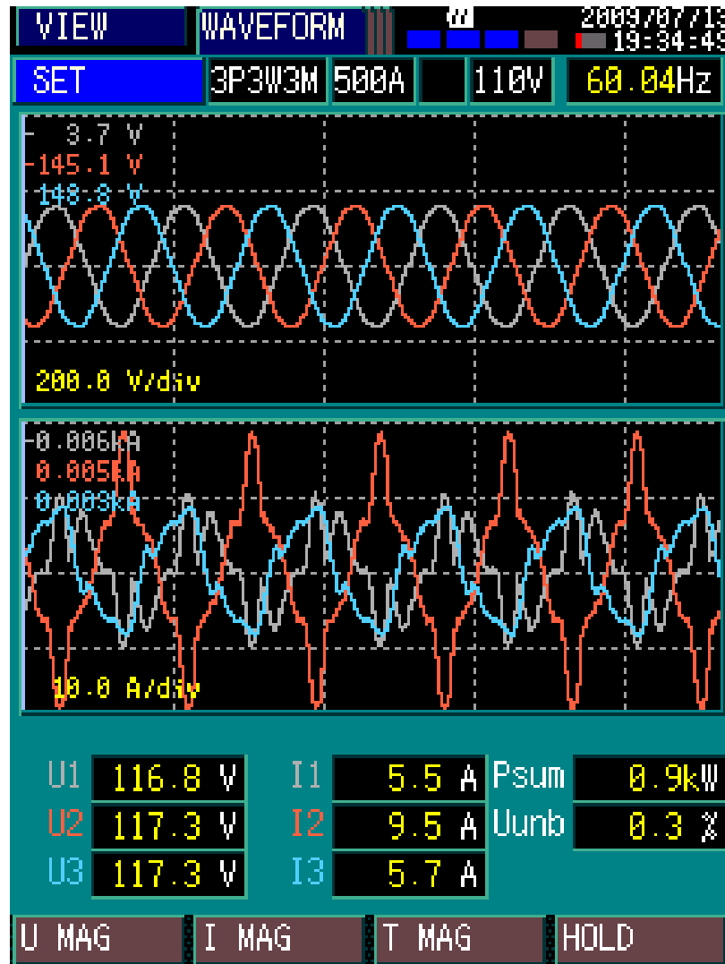
120V 3 phase lighting panel on ship
