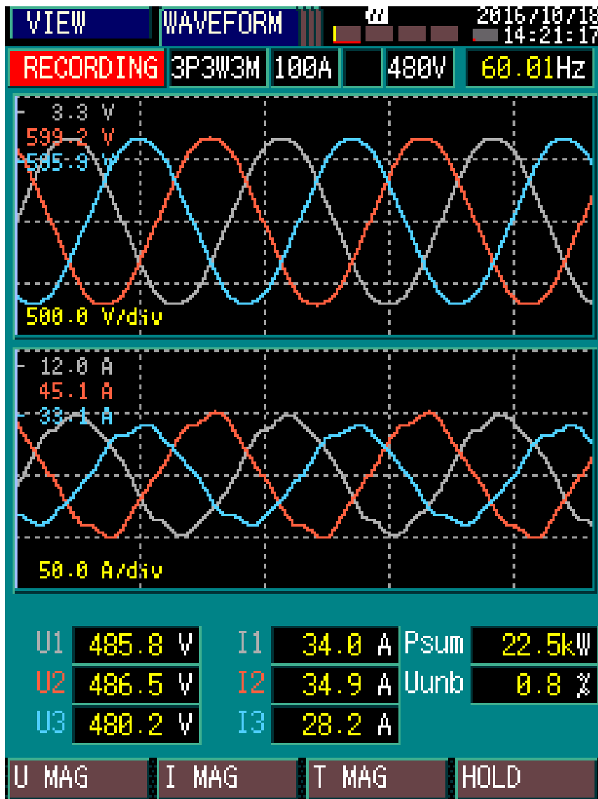
480 VAC 3 phase panel on ship
