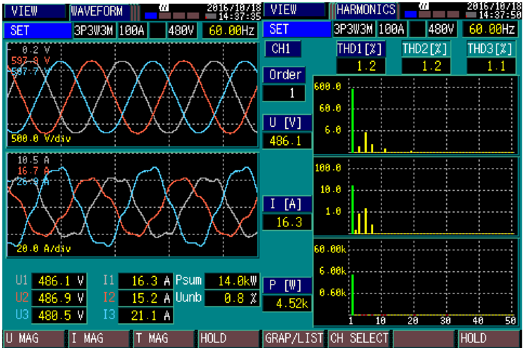
480 3 phase panel on ship
